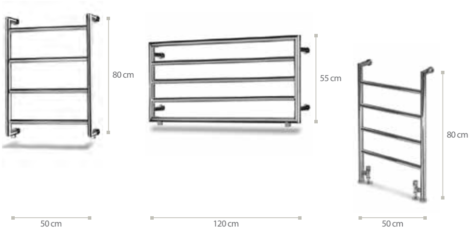
Palma 4 Watts: 266 (Delta T60)
